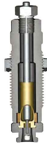
CONTOUR GROUND CARBIDE SIZING DIE
