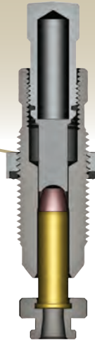
BULLET SEAT & FEED DIE
